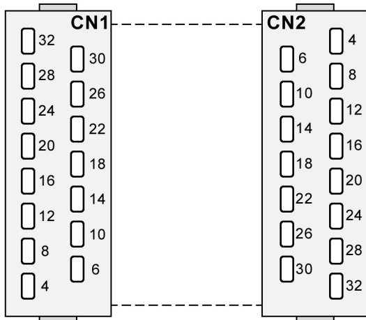
Schema connettore H15 / H15 plug-in connector wiring scheme:
